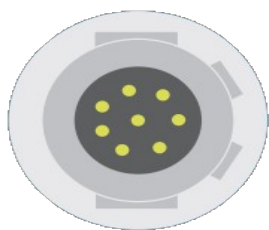
SENSOR DE CAPNOGRAFIA MAINSTREAM – RESPIRONICS CAPNOSTAT 5
